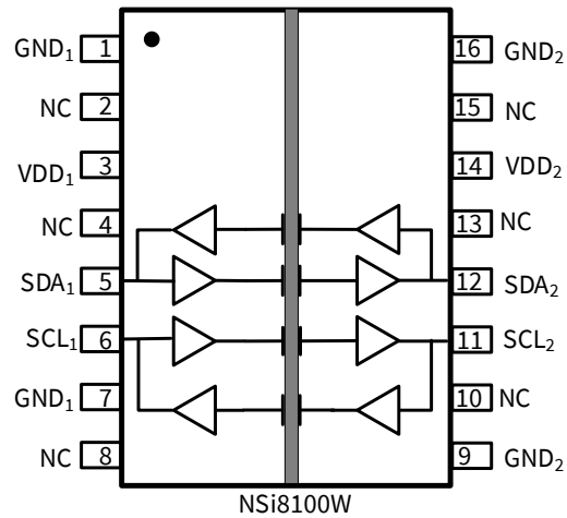
Figure 1.2 NSi8100W Package
