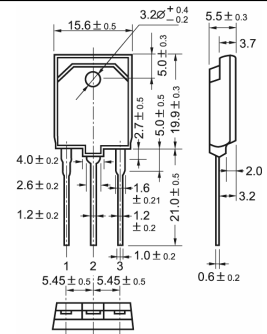
TO-3PFM
