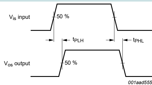
Fig. 13. Input ( V_{\text{is}} ) to output ( V_{\text{os}} ) propagation delays
