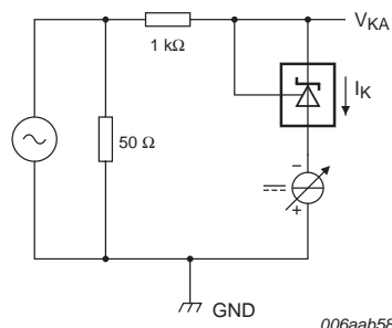
Fig 22. Test circuit to Figure 19, Figure 20 and Figure 21
