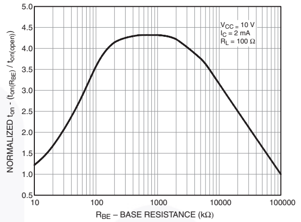
Figure 10. Normalized t_{on} vs. R_{BE}
