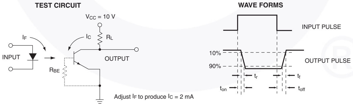
Figure 13. Switching Time Test Circuit and Waveform
