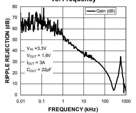
Ripple Rejection ( I_{OUT} = 3A ) vs. Frequency
