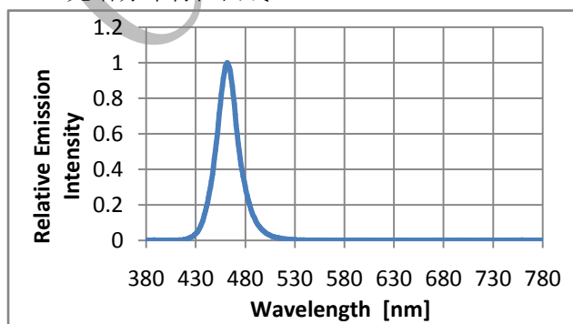
Fig.7- Spectrum Distribution
