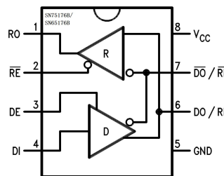
Figure 1. Top View
