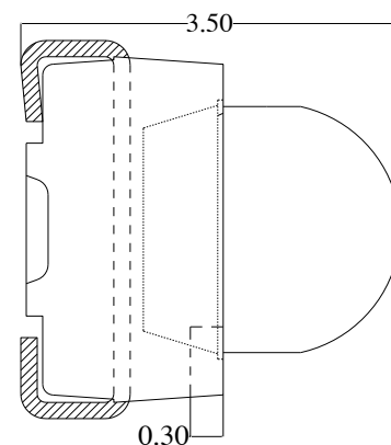
Fig.1-2 Side View 侧面视图
