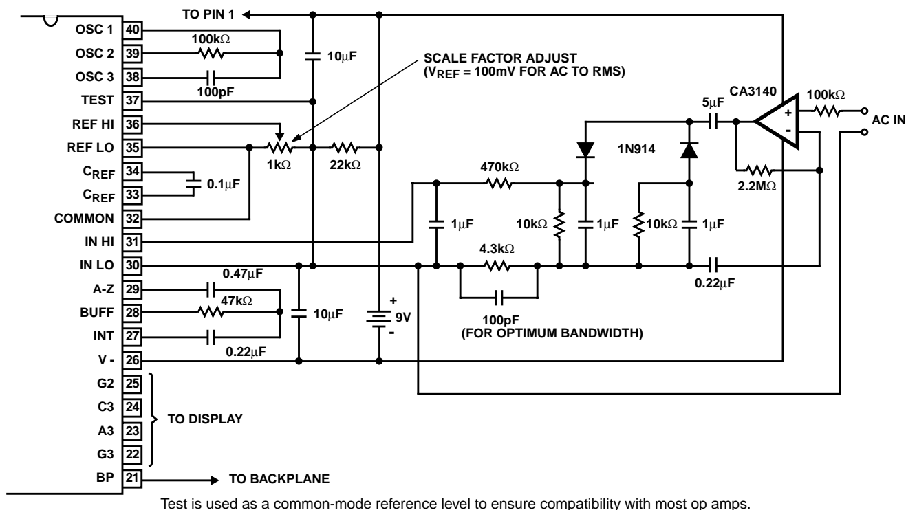
FIGURE 21. AC TO DC CONVERTER WITH WS7106
