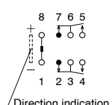
1 coil latching (Reset condition)
