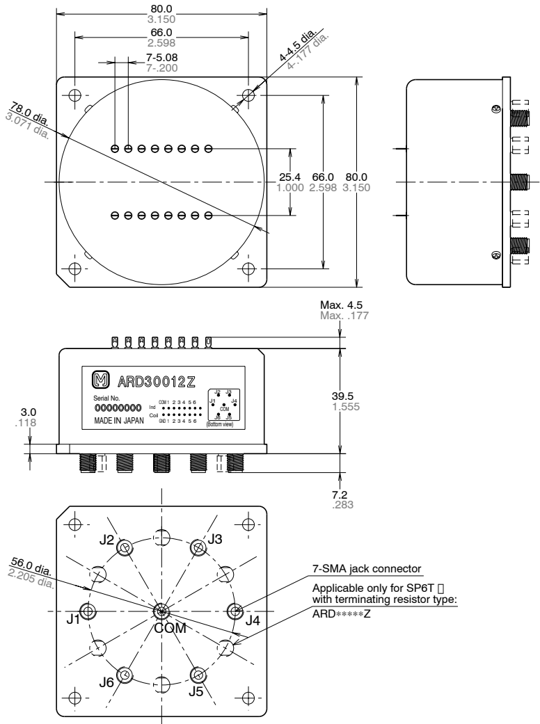
Latching type
