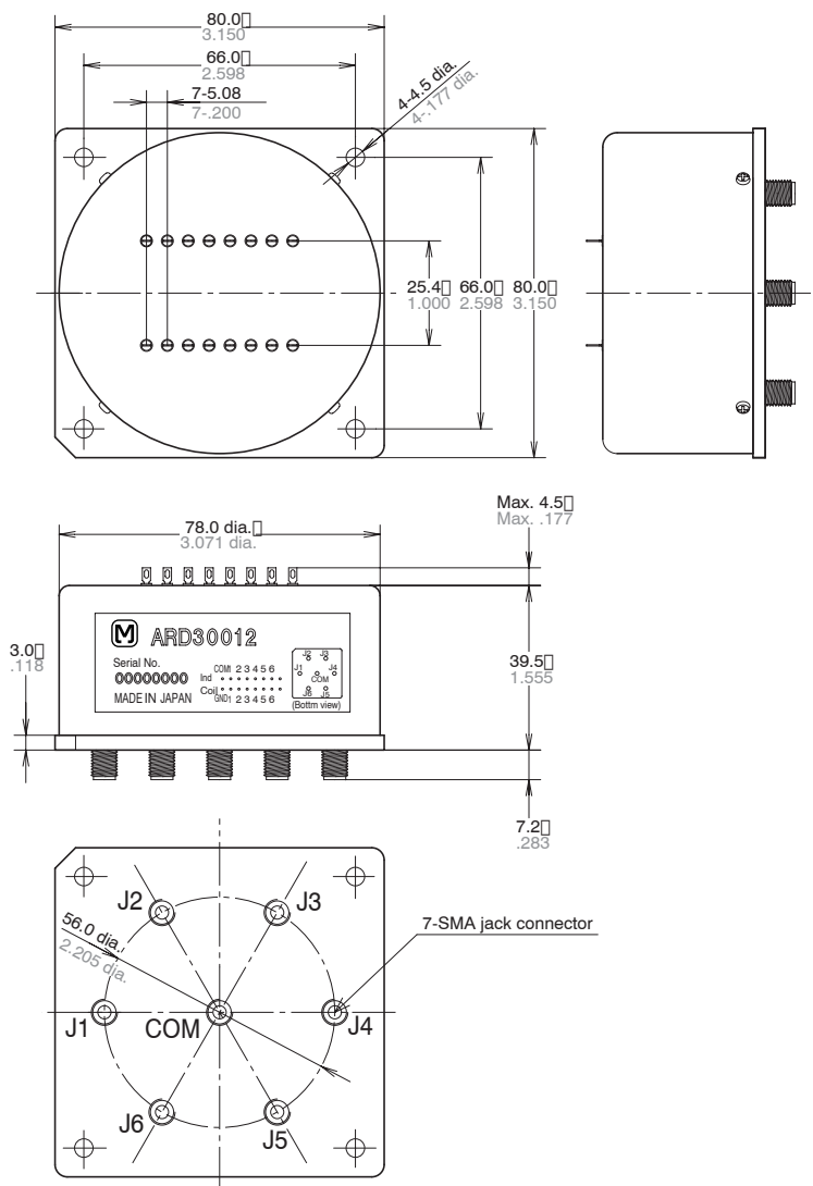
Latching type
