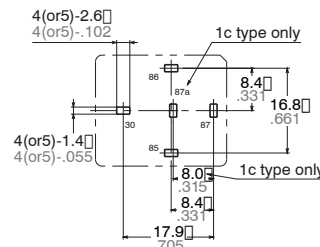
PC board pattern
