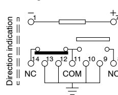
(Deenergized condition)
