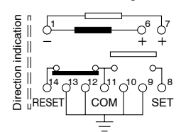
(Reset condition)
