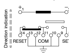
(Reset condition)
