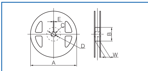
Standard Reel Dimensions
