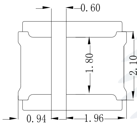
Fig.1-3 Bottom View
