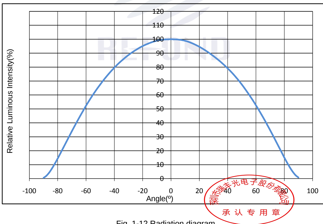
Fig. 1-12 Radiation diagram
