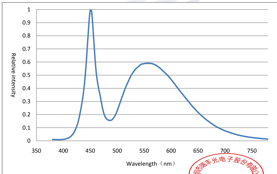
Fig. 1-14 Spectrum Distribution
