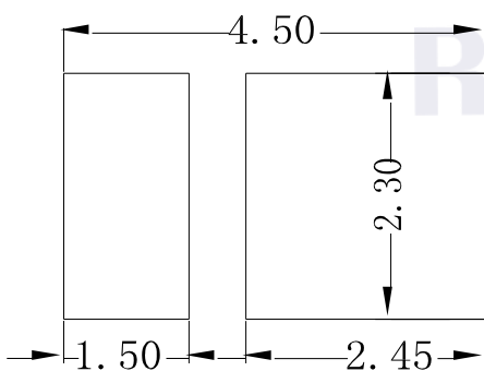
Fig.1-5 Soldering Patterns
