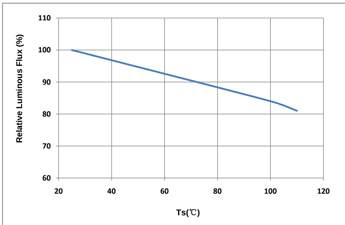
Fig. 1-9 Solder Temperature Vs Relative Intensity
