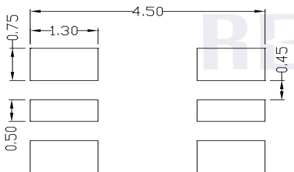
Fig. 1-5 Soldering Patterns 推荐焊盘
