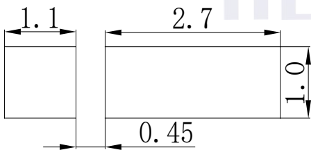
Fig. 1-5 Soldering Patterns 推荐焊盘
