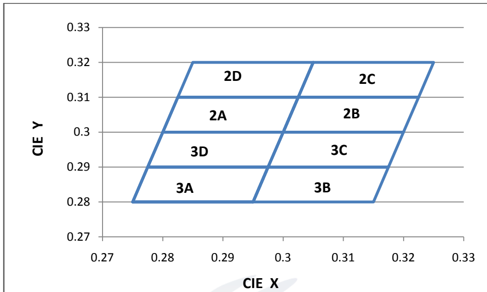
Fig 1-6 The C.I.E Chromaticity Diagram CIE色度图
