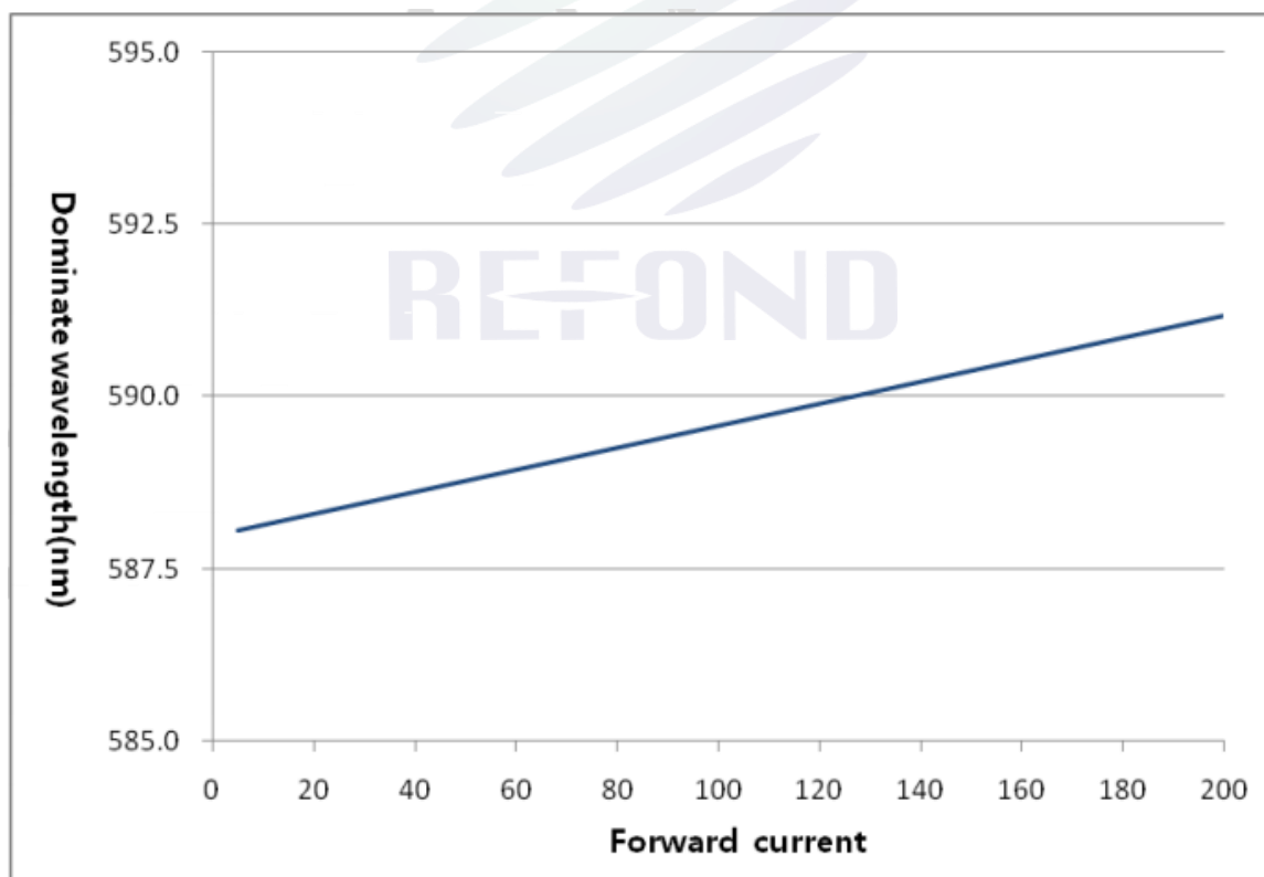
Fig. 1-12 Forward current vs. Dominate wavelength 正向电流与主波长特性曲线 ( T_s=25^\circ\text{C} )
