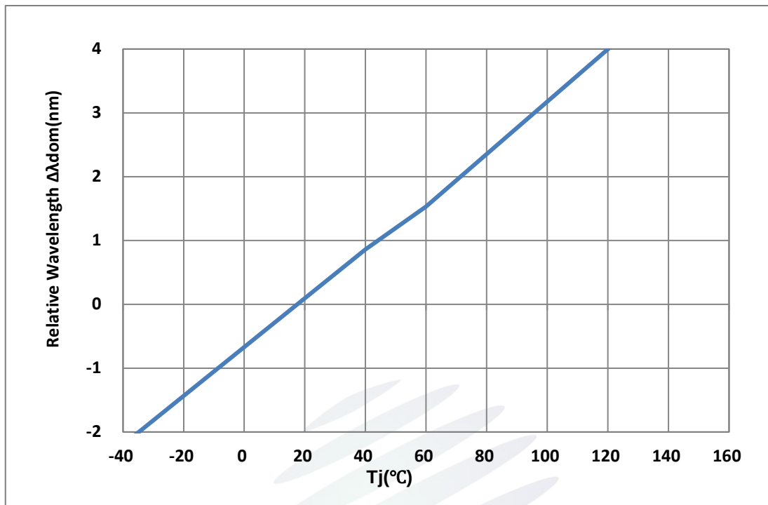
Fig. 1-13 Dominant Wavelength Shift Vs Junction Temperature 波长偏移与结温特性曲线
