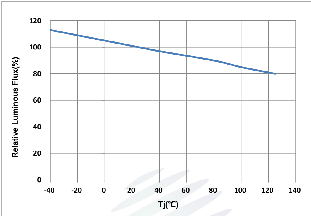
Fig. 1-9 Junction Temperature Vs Relative flux结温与相对光通量特性曲线
