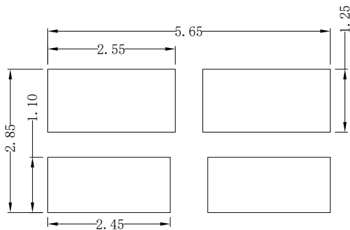
Fig.1-5 Soldering Patterns 推荐焊盘
