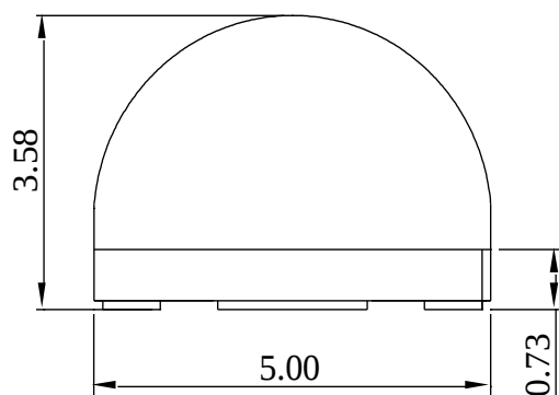
Fig.1-2 Side view 侧面视图
