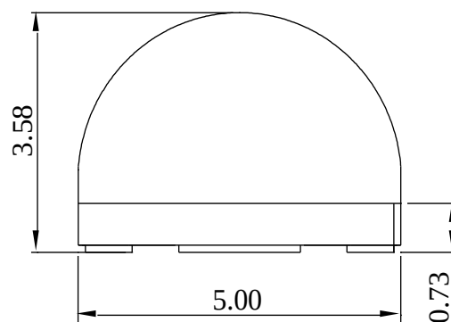
Fig.1-2 Side view 侧面视图
