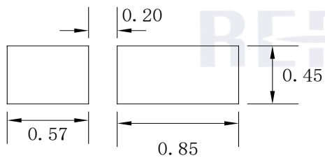
Fig. 1-5 Soldering Patterns 推荐焊盘
