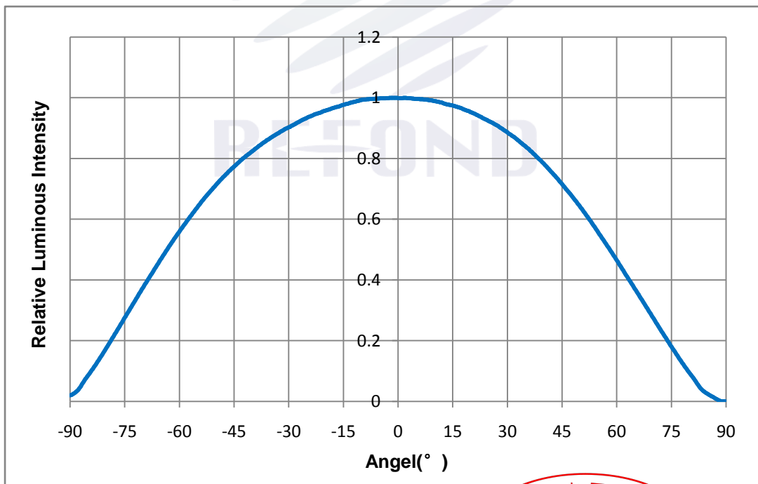
Fig 1-12 Radiation diagram
