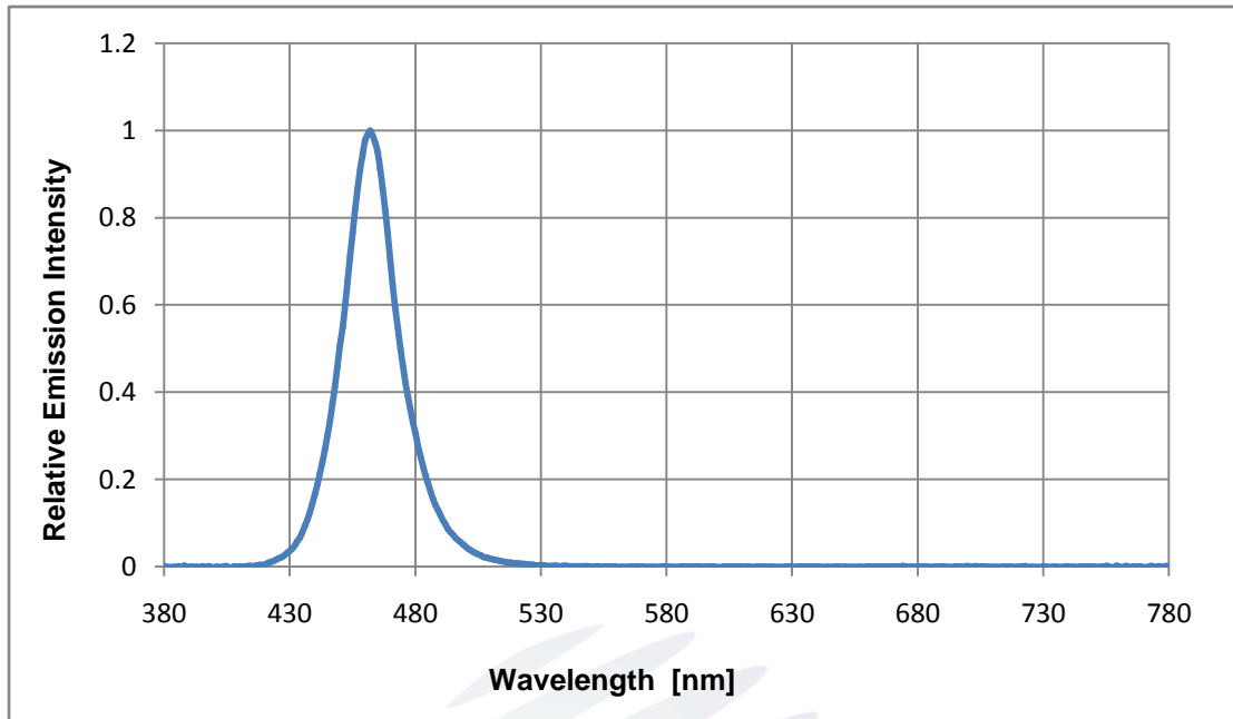
Fig 1-13 Spectrum Distribution
