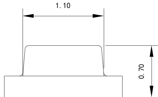
Fig.1-2 Side view
