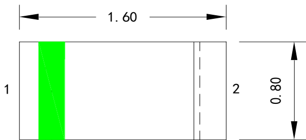
Fig.1-1 Top view
