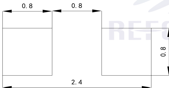
Fig.1-5 Soldering patterns
