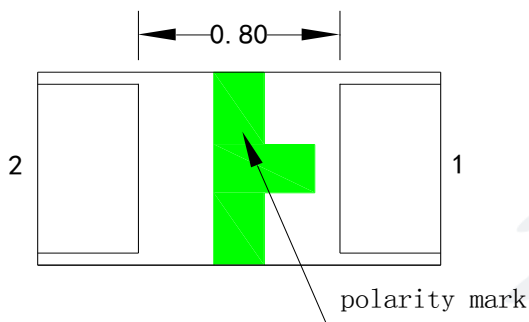
Fig.1-3 Bottom view
