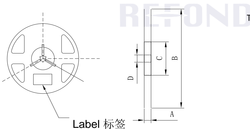
Fig.2-2 Reel Dimension 卷盘尺寸
