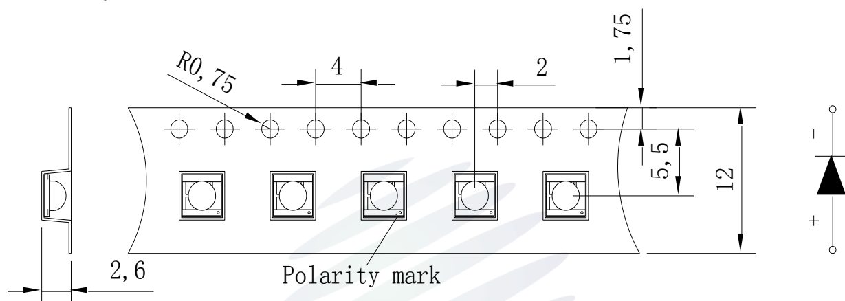
Fig.2-1 Carrier Tape Dimension 載帶尺寸
