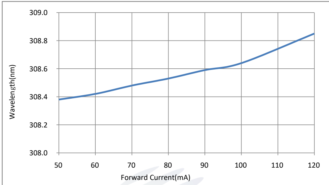
Fig.1-8 Peak Wavelength Vs. Forward Current 正向电流与峰值波长曲线
