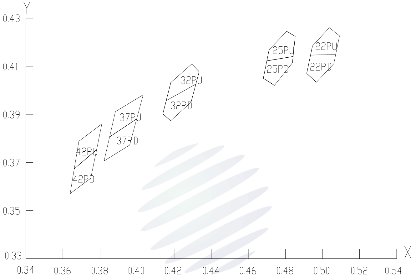
Fig 1-6 The C.I.E Chromaticity Diagram
