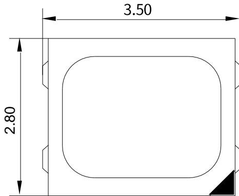
Fig.1-1 Top view
