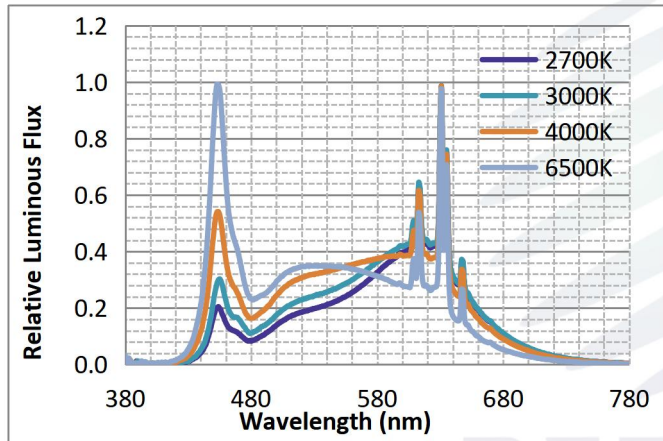
Typical spectrum distribution 典型光谱分布 ( T_s=25^\circ\text{C} IF=150mA)
