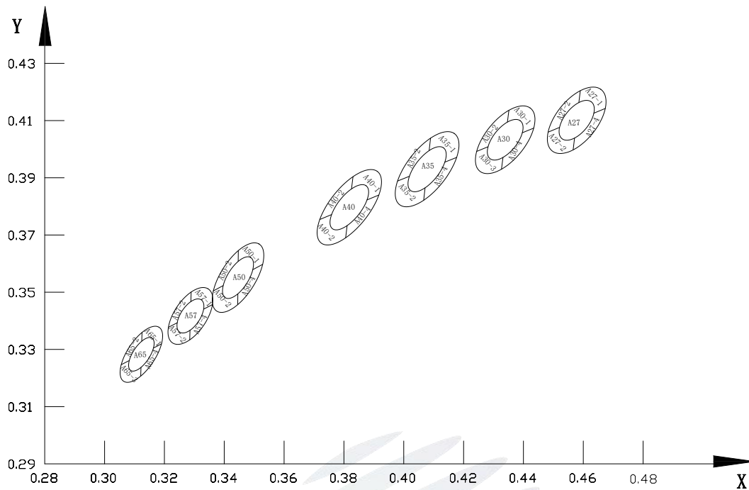
Fig 1-6 The C.I.E Chromaticity Diagram CIE色度
