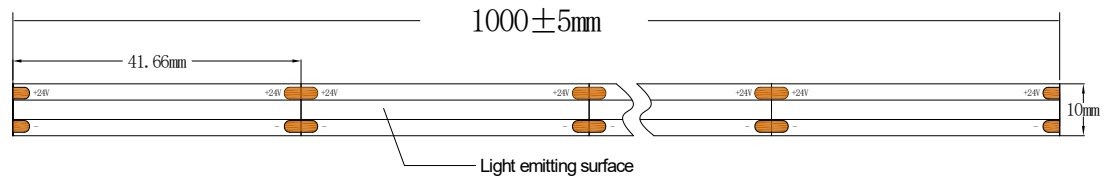
Fig.1-1 FPC board size drawing FPC 板尺寸
