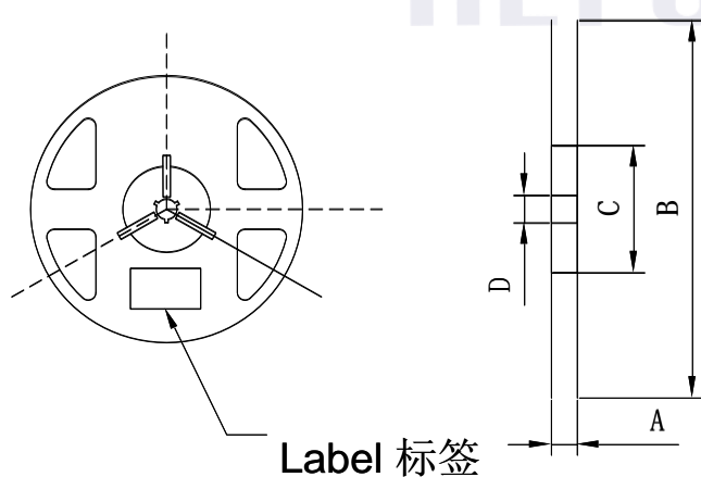
Fig.2-2 Reel 卷盘
