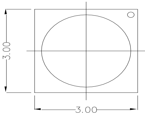
Fig.1-1 Top view
