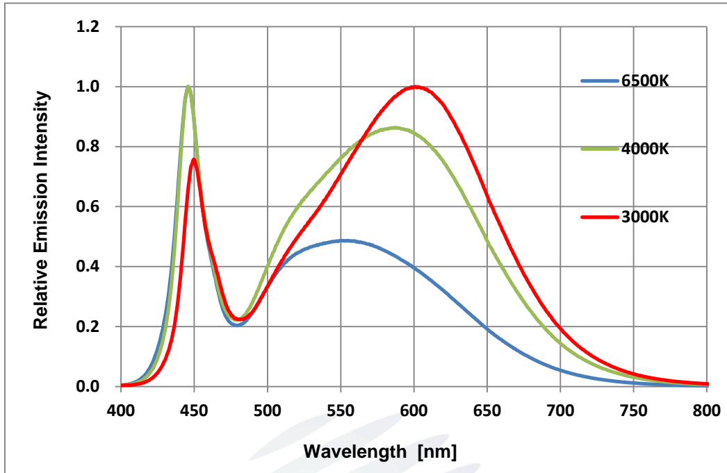
Fig 1-13 Spectrum Distribution
