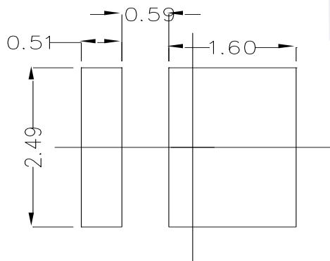
Fig.1-5 Soldering patterns
