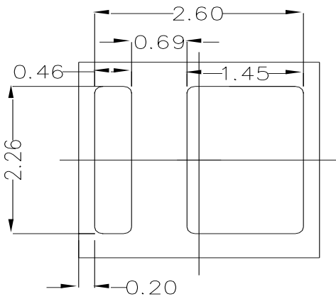
Fig.1-3 Bottom view
