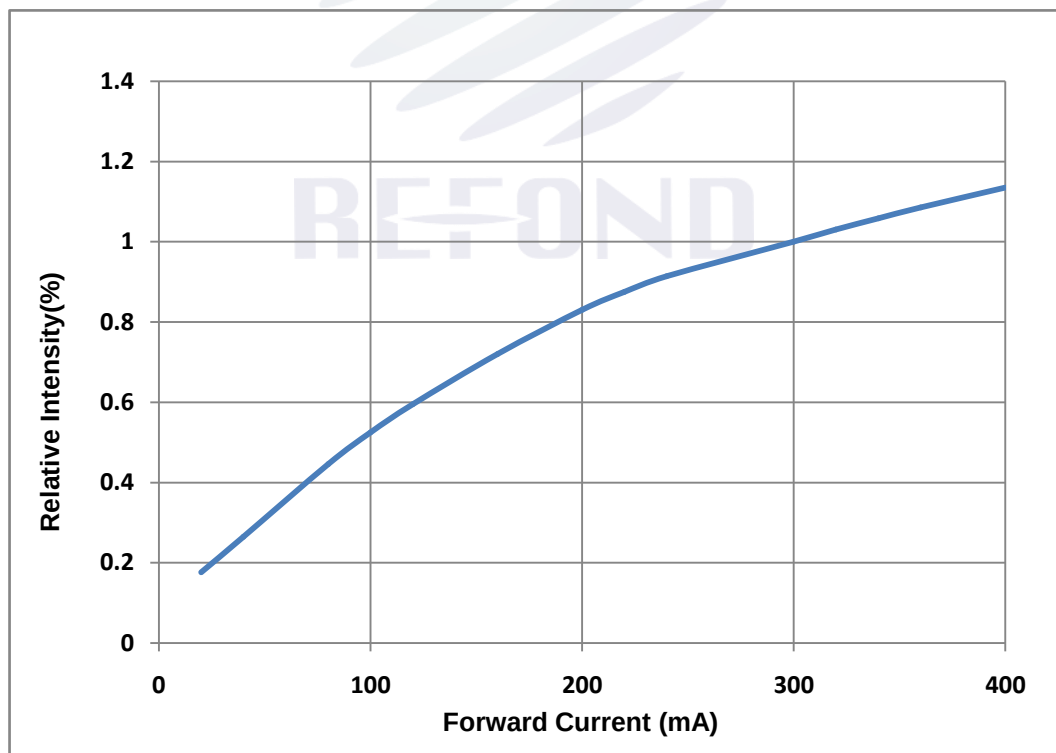
Fig 1-8 Forward Current Vs. Relative Intensity 正向电流与相对光强特性曲线 T_s=25^{\circ}\text{C}
