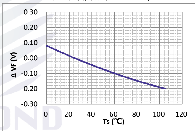
Forward voltage vs. Ts temperature 电压与温度曲线 (IF=800mA)
