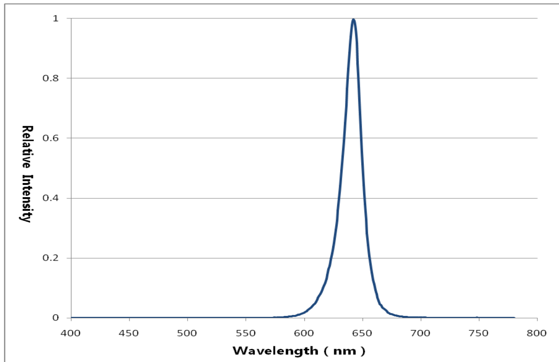
Fig.5 Relative Intensity vs. Wavelength (Ts=25°C)
