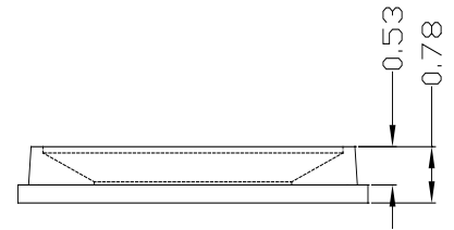
Fig.1-2 Side view 侧面视图
