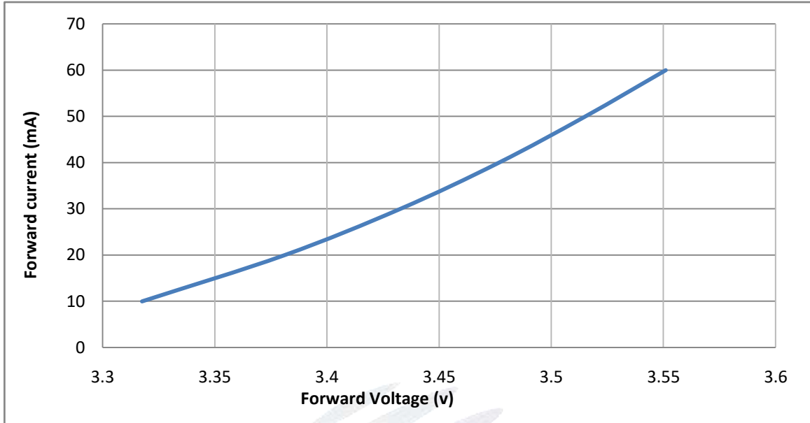
Fig 1- Forward Voltage Vs. Forward Current 伏安特性曲线
