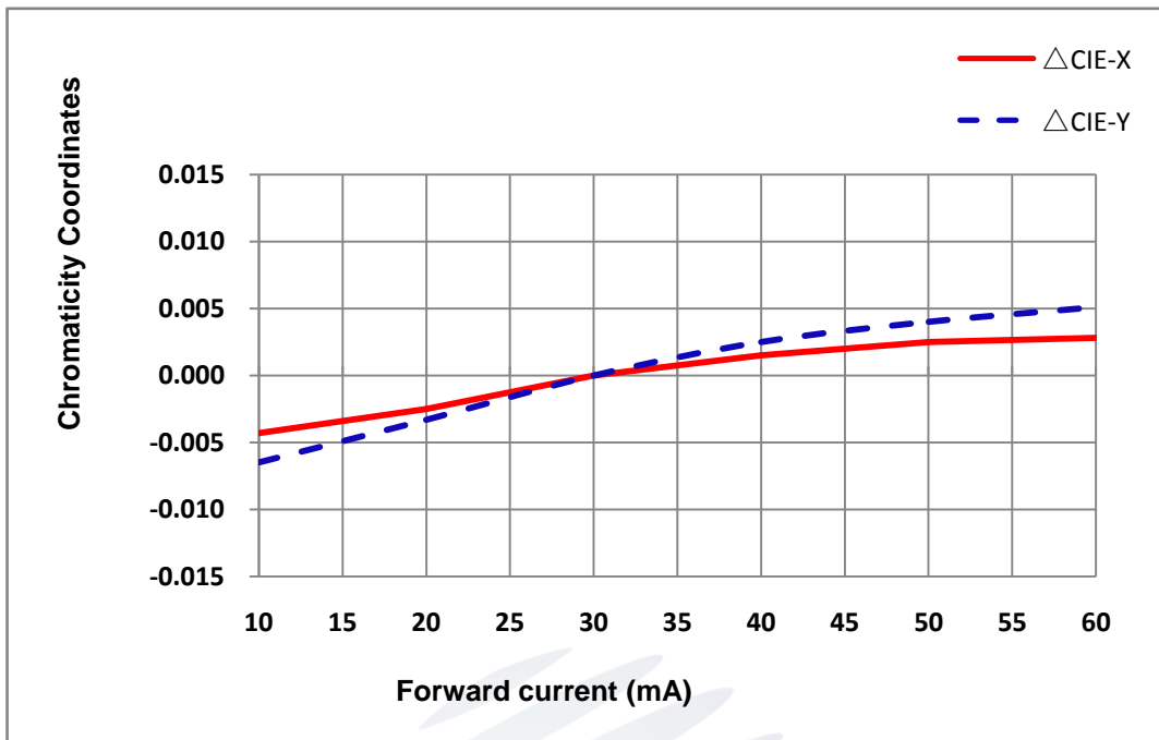
Fig. 1-13 Chromaticity Coordinate Shift Vs Forward Current 色坐标与电流特性曲线
