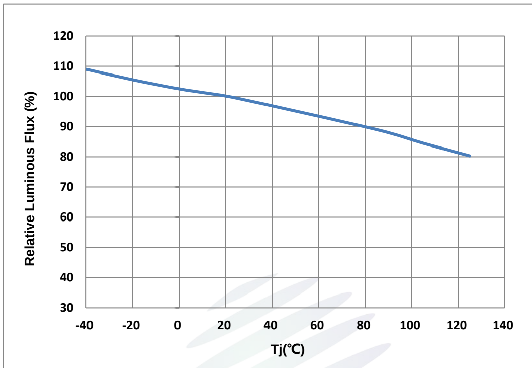
Fig. 1-9 Junction Temperature Vs Relative Intensity结温与相对光通量特性曲线
