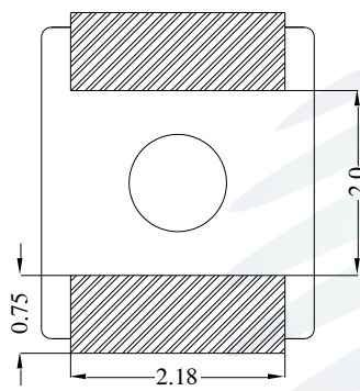
Fig.1-3 Bottom View
