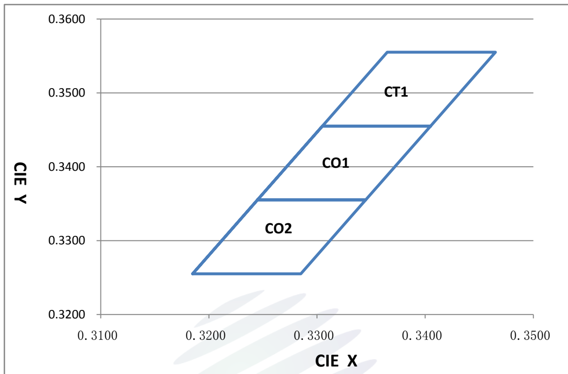
Fig. 1-6 The C.I.E Chromaticity Diagram
