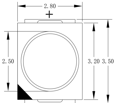
Fig.1-1 Top View
