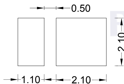
Fig.1-5 Soldering patterns 推荐焊盘
