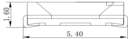
Fig.1-2 Side view 侧面视图
