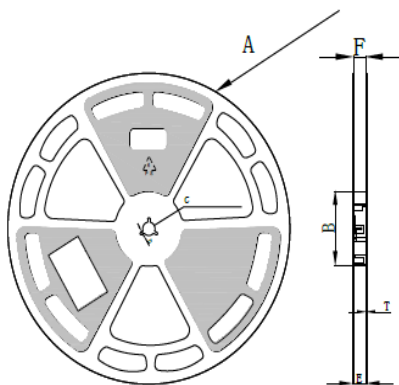
Fig.2-2 Reel 卷盘
