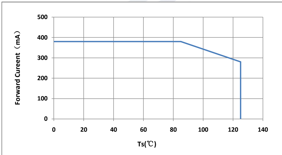
Fig. 1-10 Solder Temperature Vs Forward Current 管脚温度与正向电流特性曲线 T j ≤ 150°C
