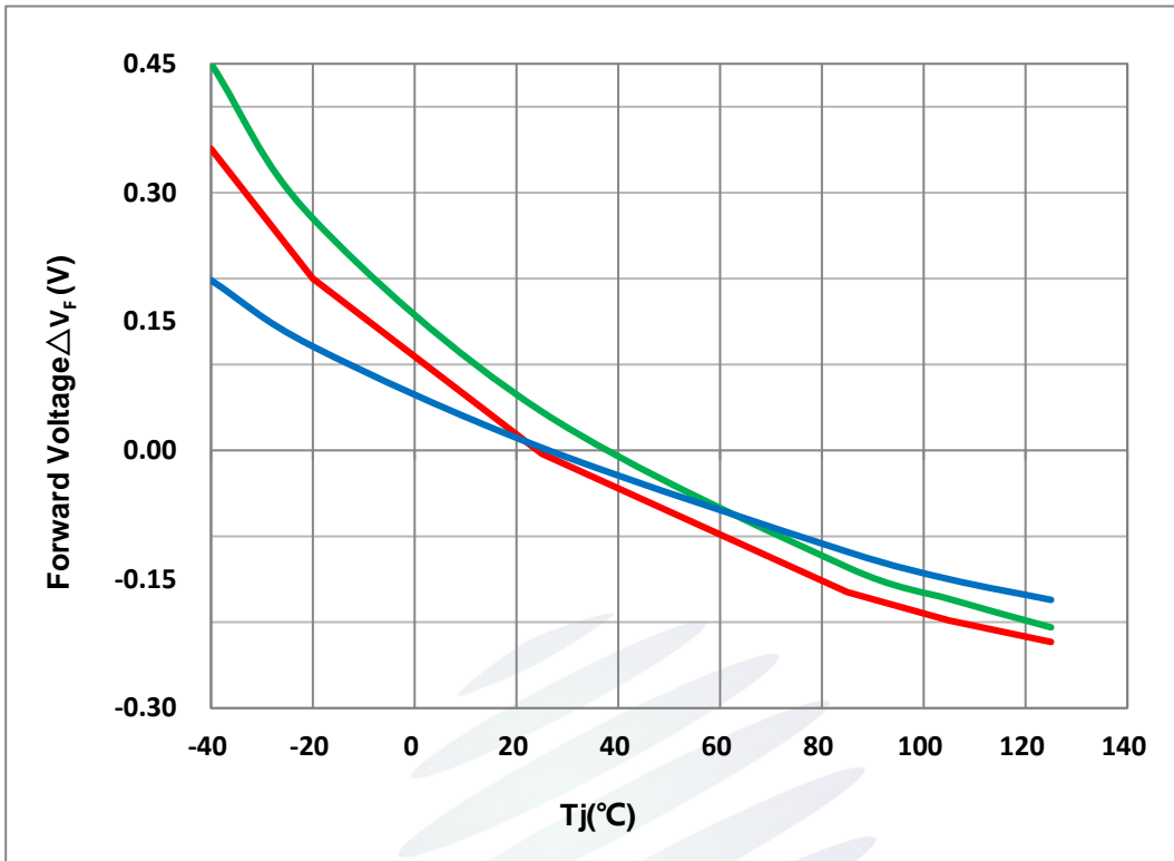
Fig. 1-11 Voltage Shift Vs Junction Temperature 电压偏移与结温特性曲线
