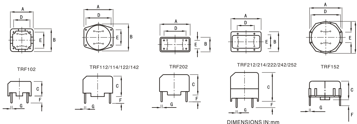
DIMENSIONS IN:mm
