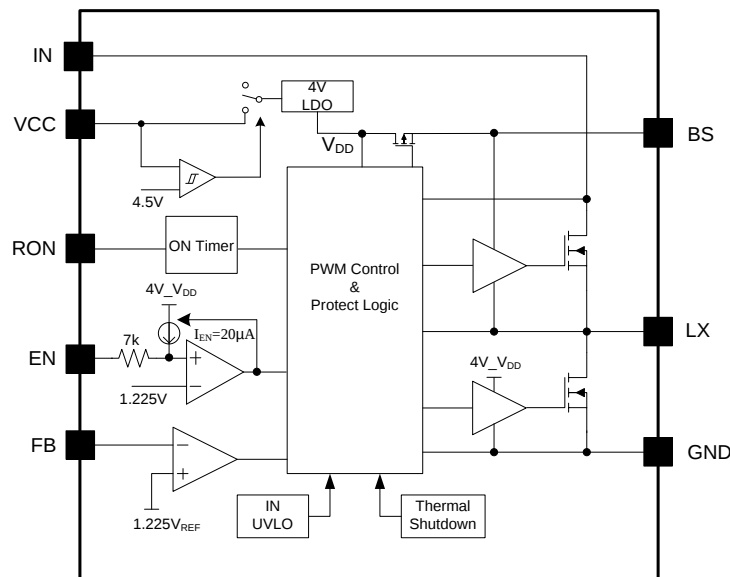
Figure3. Block Diagram
